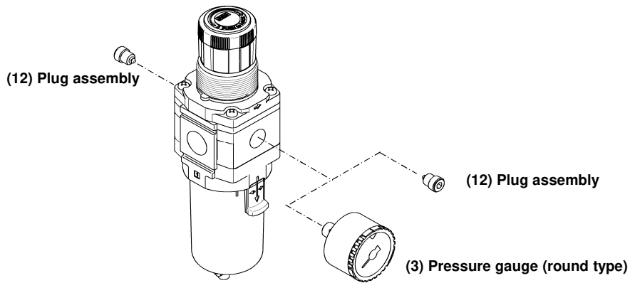
Micro mist separator regulator
