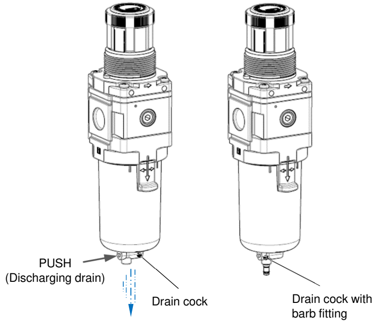
AWD30-D/ AWD40-D: Drain cock/ With barb fitting (push type) (Polycarbonate bowl/ Nylon bowl)
