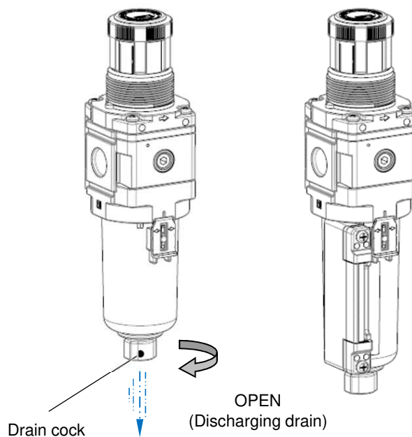
AWD30-D/ AWD40-D: Drain cock (rotation type) (Metal bowl/ Metal bowl with level gauge)
