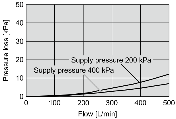
PF2MC7501 (500 L/min)
