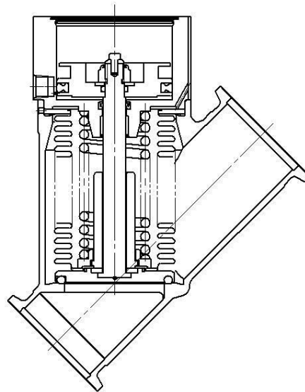
XYC series / Straight Valve
