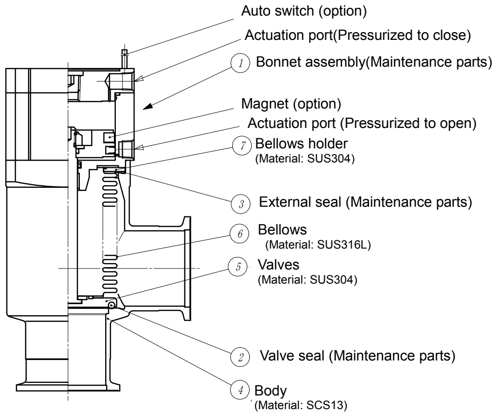
XMC series / Angled Valve
