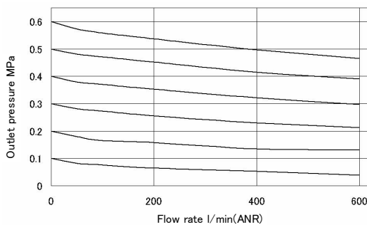
AR30-X2400
