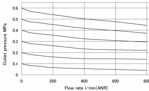
Rc 3/8
