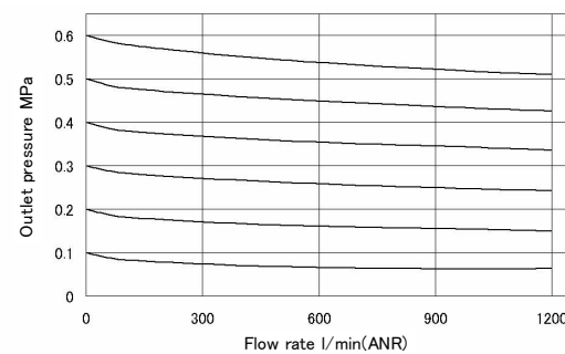
Rc 3/4
