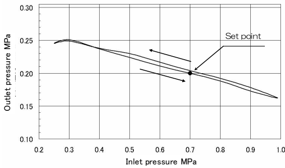
AR50-X2400
