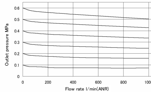
Rc 3/8
