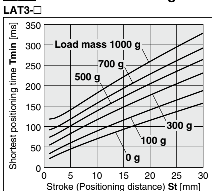
Fig. 3 Shortest Positioning Time (Reference): T_{min} [ms]
