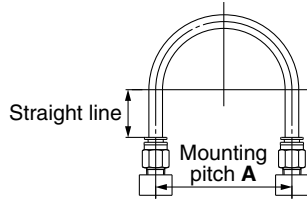
Fig. 1 Recommended piping
