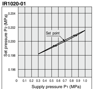
IR1020-01 Back pressure: 1.0 MPa
