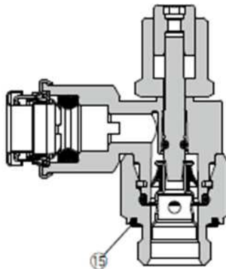
Meter-out
