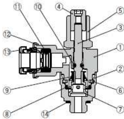
Meter-out
