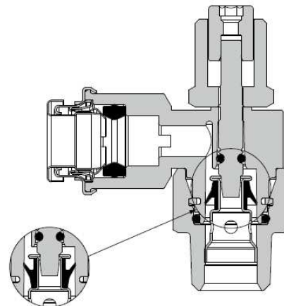
Meter-In
