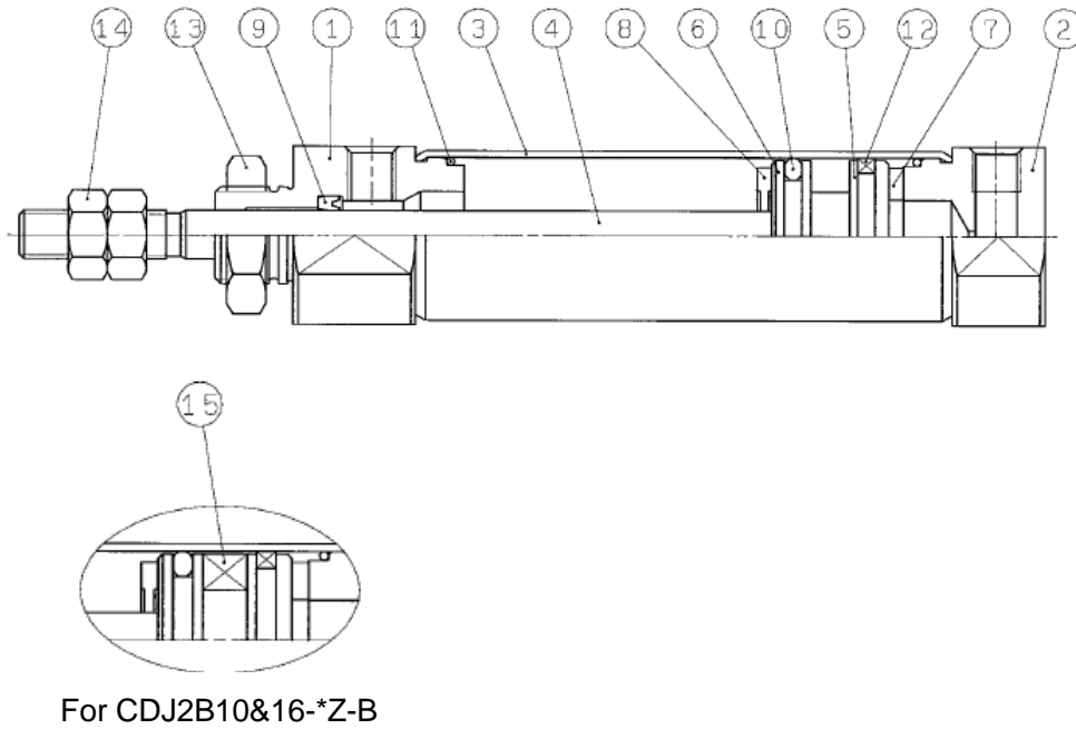
Fig. 4 Standard product: Double acting/single rod
