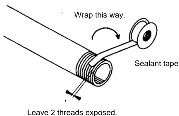
Fig. 2 Sealant tape
