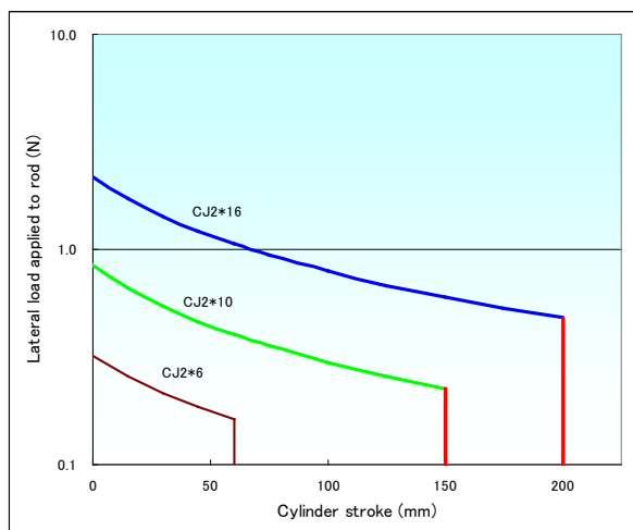
Fig. 1 Allowable lateral load applied to rod end
