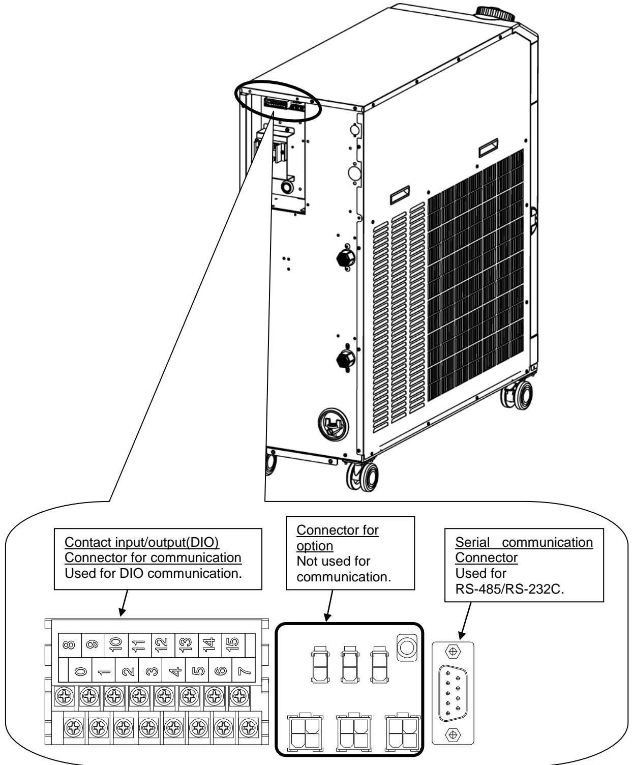
Fig 1.2-1 Communication port
