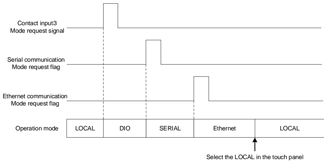
Fig. 1-1 Mode switching by the mode request (Standard)
