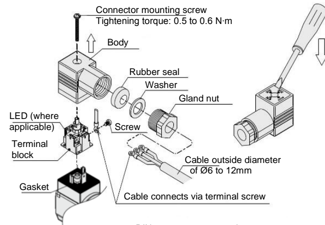
Figure 7. DIN connector construction
