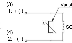
Figure 11. Grommet / DIN terminal / Conduit with surge voltage suppressor / M12 connector (3,4)
