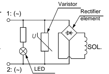
Figure 14. DIN terminal with LED and surge voltage suppressor
