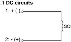
Figure 10. Grommet without electrical option
